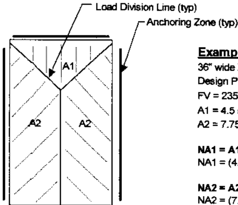
Single Door
