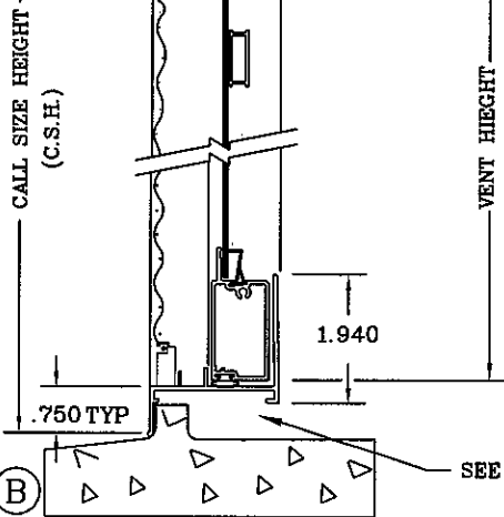
HEADER AND SILL SECTION TYP. 1 BY BUCK
