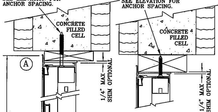
ALT. HEADER SECTION TYP. 2 BY BUCK
