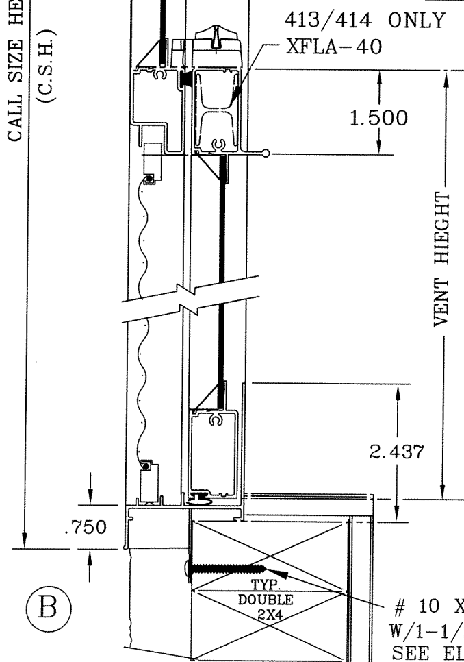
HEADER AND SILL SECTION WOOD FRAME
