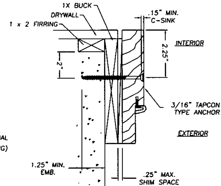
4 VERTICAL SIDE JAMB TO 1X SUB-BUCK
