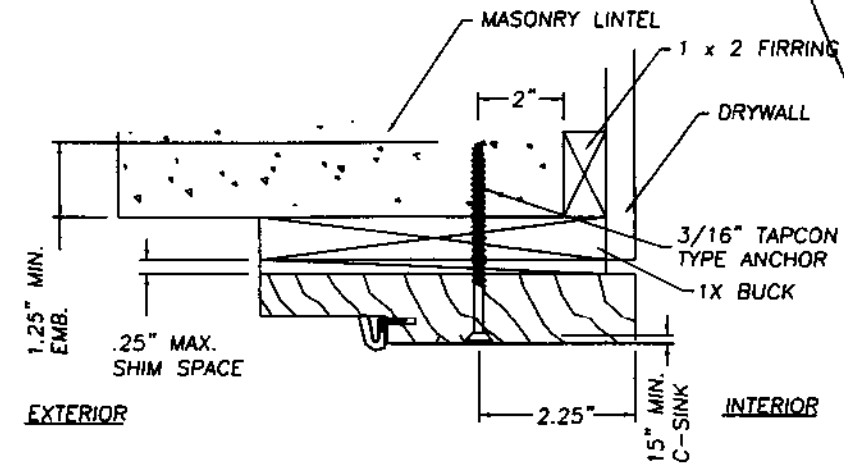
3 HEAD JAMB TO 1X SUB-BUCK
