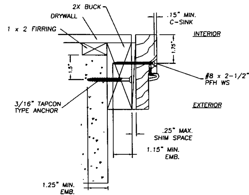
2 VERTICAL SIDE JAMB TO 2X SUB-BUCK
