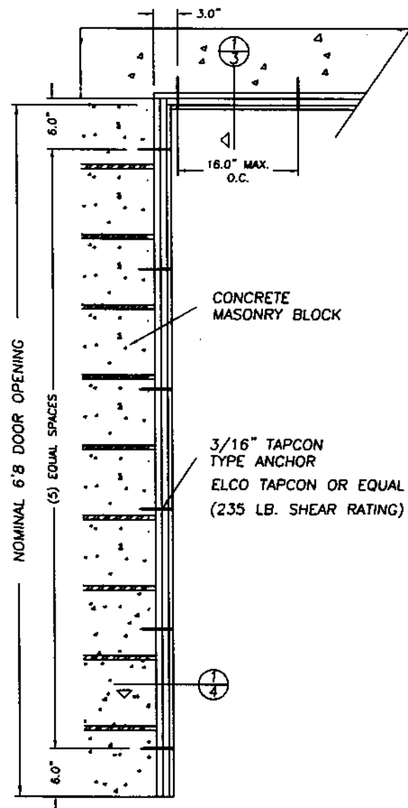
1 X INSTALLATION
