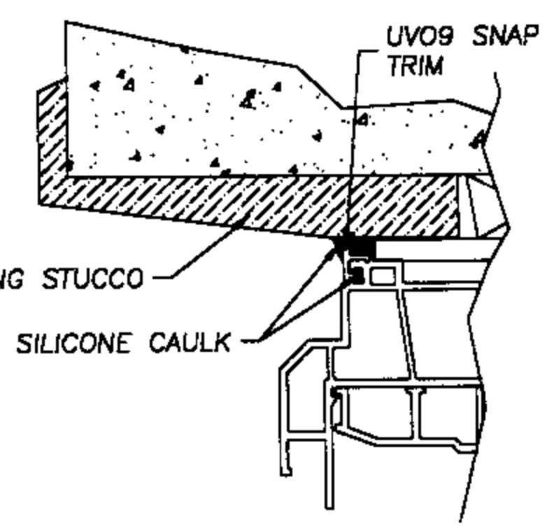
DETAIL "A" UVO9 SNAP TRIM DETAIL SEE NOTE 5
