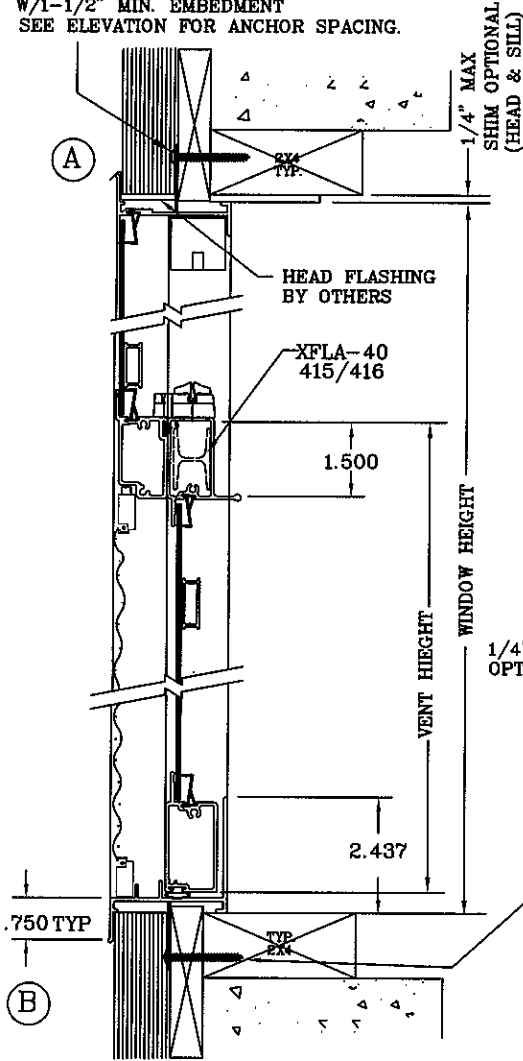
HEADER AND SILL SECTION
