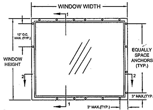
ELEVATION VIEWED FROM EXTERIOR
